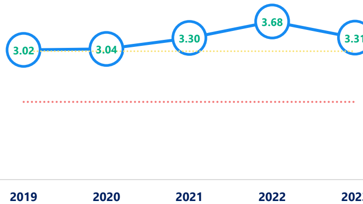
Z - Score
